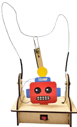
Hand steadiness circuit (Buzz Wire)
