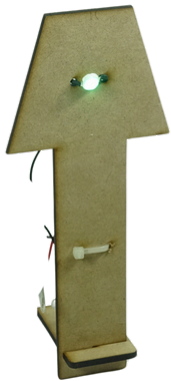
Tilt Switch Design
